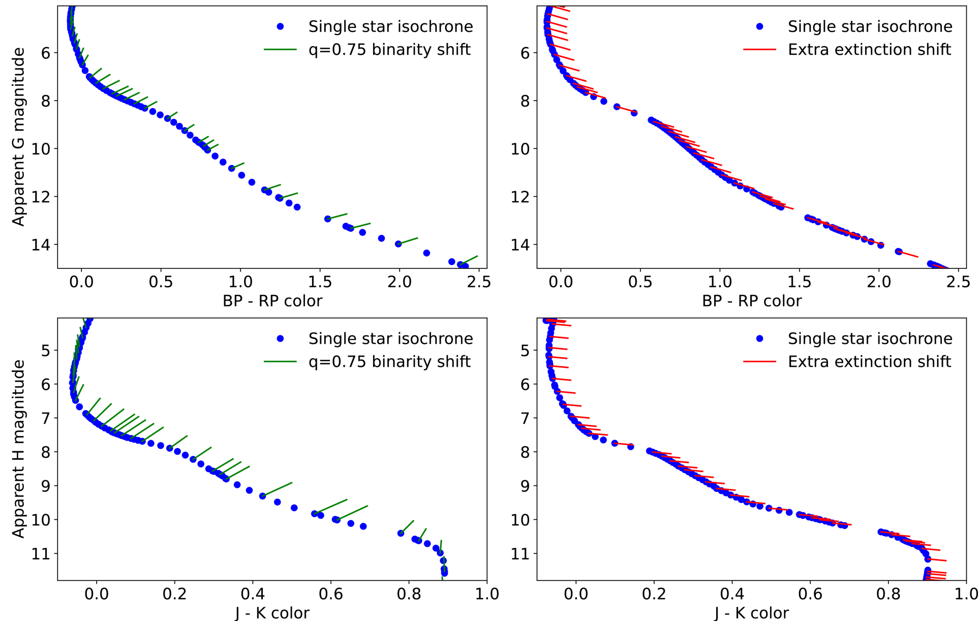
Figure 6. from Dmitry Chulkov 2026 Astron. J. 171 doi:10.3847/1538-3881/ae284e https://dx.doi.org/10.3847/1538-3881/ae284e © 2026. The Author(s). Published by the American Astronomical Society.
