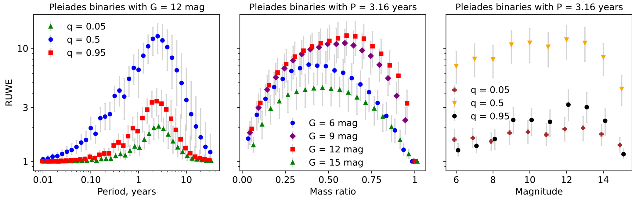
Figure 3. from Dmitry Chulkov 2026 Astron. J. 171 doi:10.3847/1538-3881/ae284e https://dx.doi.org/10.3847/1538-3881/ae284e © 2026. The Author(s). Published by the American Astronomical Society.
