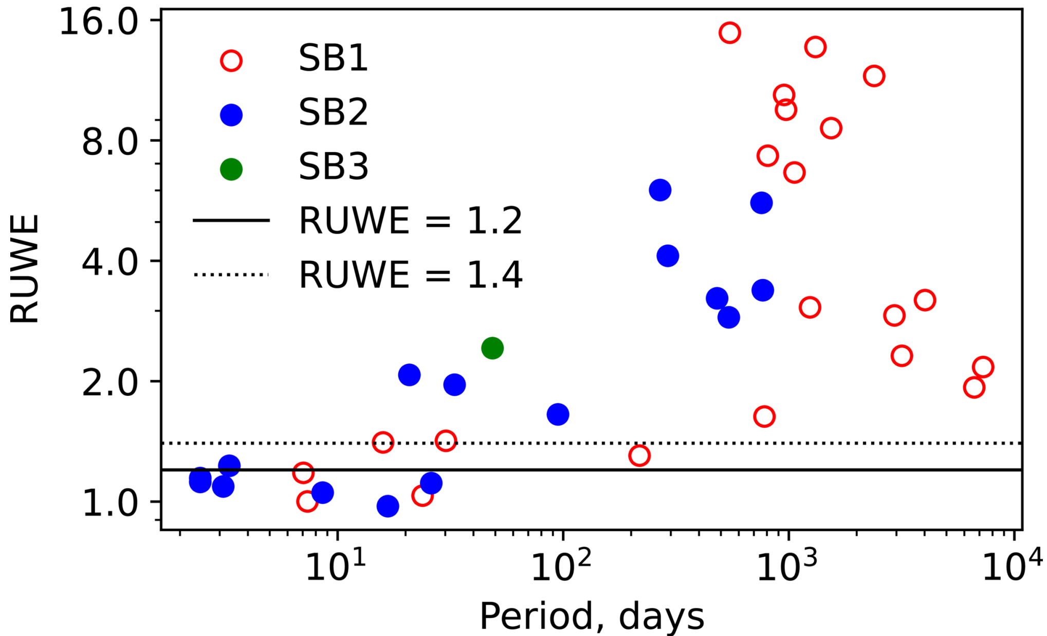
Figure 1. from Dmitry Chulkov 2026 Astron. J. 171 doi:10.3847/1538-3881/ae284e https://dx.doi.org/10.3847/1538-3881/ae284e © 2026. The Author(s). Published by the American Astronomical Society.
