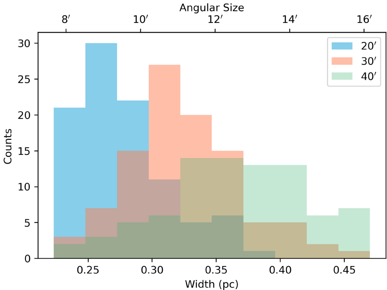
Figure 8. from M. E. Putman et al 2026 Astron. J. 171 doi:10.3847/1538-3881/ae27c3 https://dx.doi.org/10.3847/1538-3881/ae27c3 © 2026. The Author(s). Published by the American Astronomical Society.
