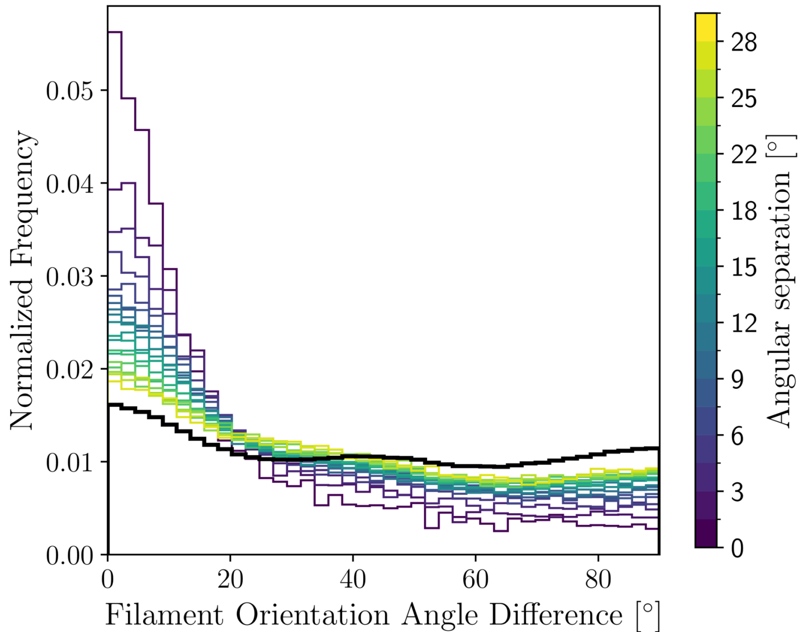
Figure 4. from M. E. Putman et al 2026 Astron. J. 171 doi:10.3847/1538-3881/ae27c3 https://dx.doi.org/10.3847/1538-3881/ae27c3 © 2026. The Author(s). Published by the American Astronomical Society.
