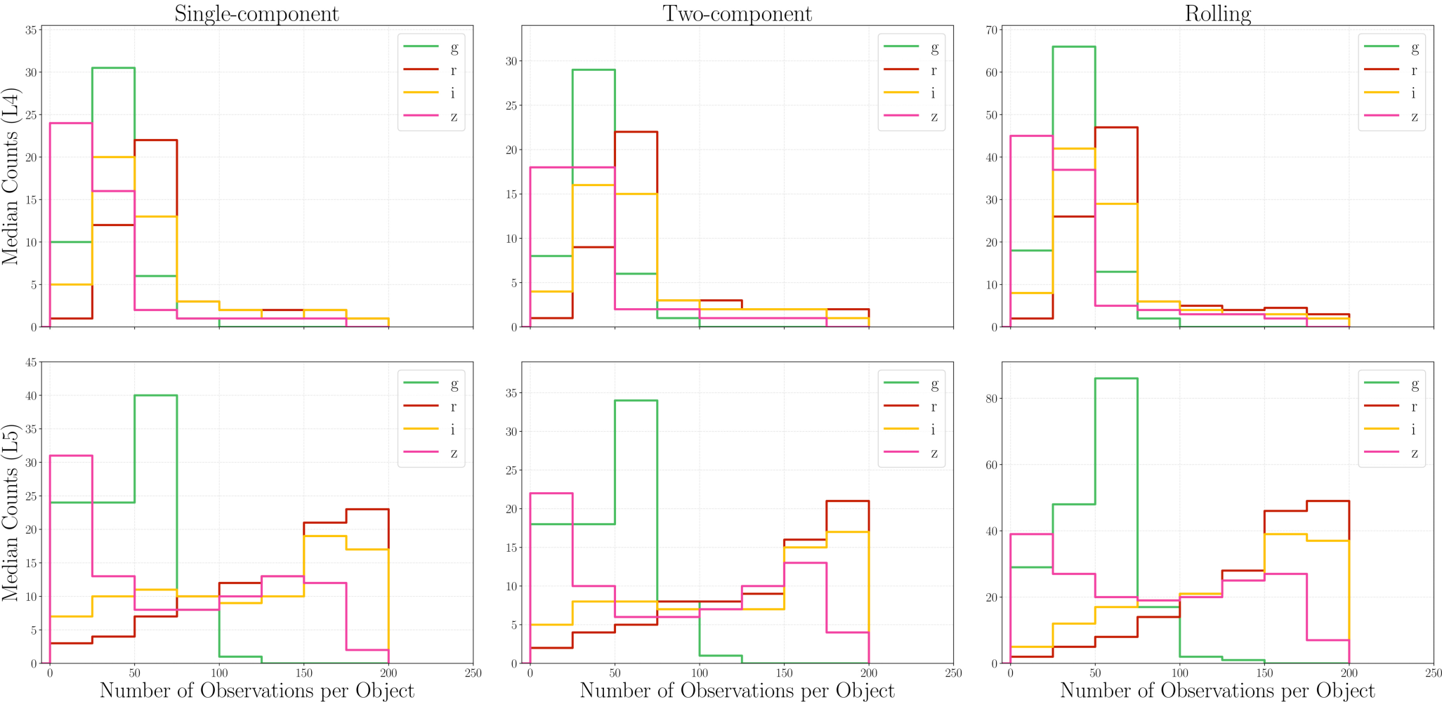
Figure 9. from Joseph Murtagh et al 2026 Astron. J. 171 doi:10.3847/1538-3881/ae27bd https://dx.doi.org/10.3847/1538-3881/ae27bd © 2026. The Author(s). Published by the American Astronomical Society.
