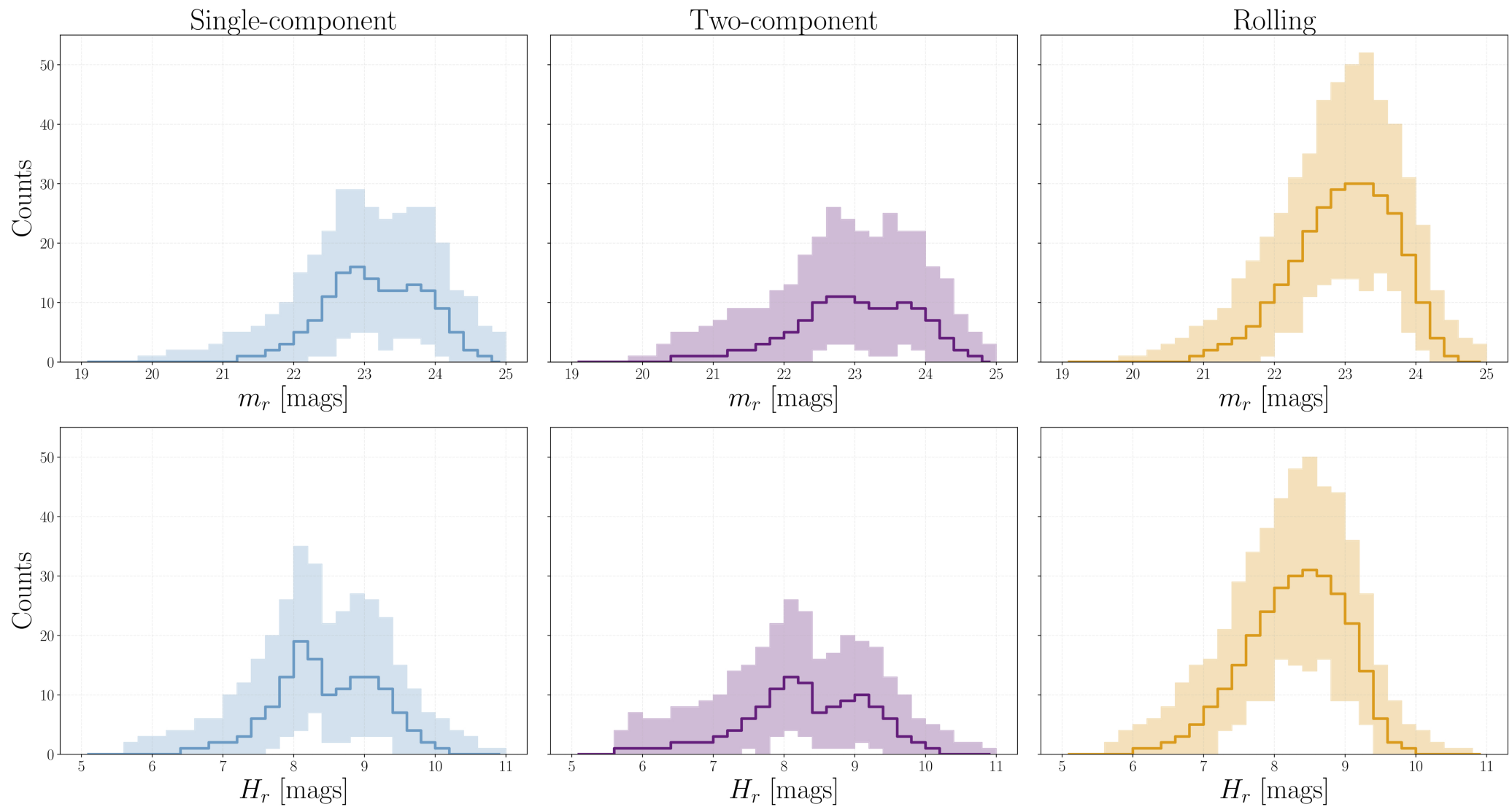
Figure 8. from Joseph Murtagh et al 2026 Astron. J. 171 doi:10.3847/1538-3881/ae27bd https://dx.doi.org/10.3847/1538-3881/ae27bd © 2026. The Author(s). Published by the American Astronomical Society.
