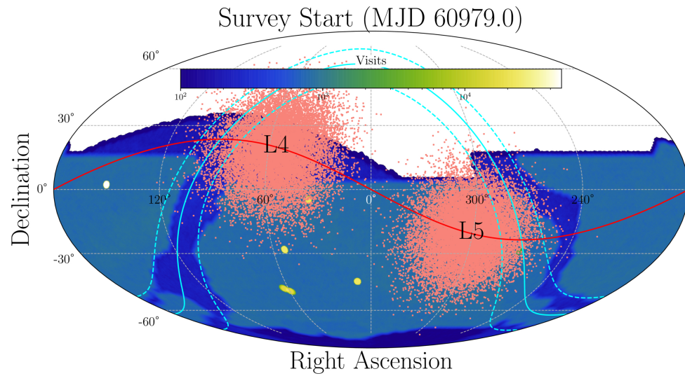
Figure 7. from Joseph Murtagh et al 2026 Astron. J. 171 doi:10.3847/1538-3881/ae27bd https://dx.doi.org/10.3847/1538-3881/ae27bd © 2026. The Author(s). Published by the American Astronomical Society.
