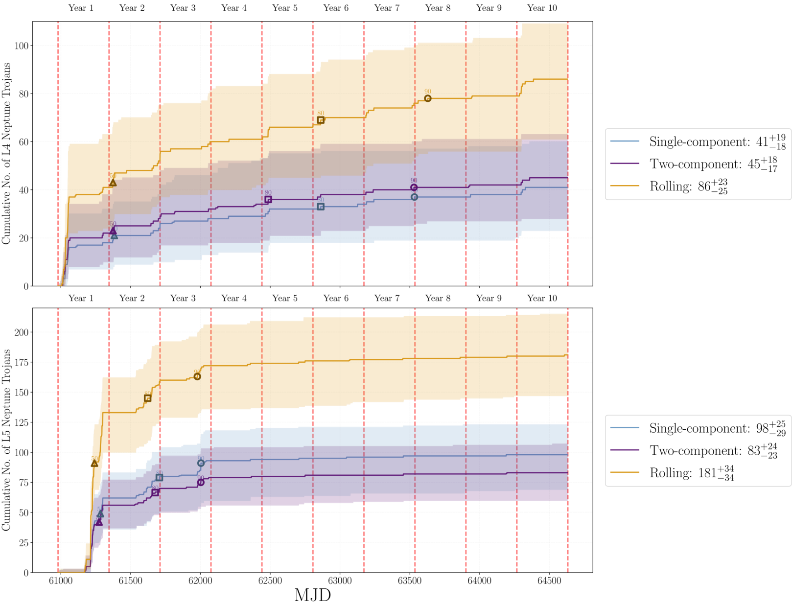
Figure 6. from Joseph Murtagh et al 2026 Astron. J. 171 doi:10.3847/1538-3881/ae27bd https://dx.doi.org/10.3847/1538-3881/ae27bd © 2026. The Author(s). Published by the American Astronomical Society.
