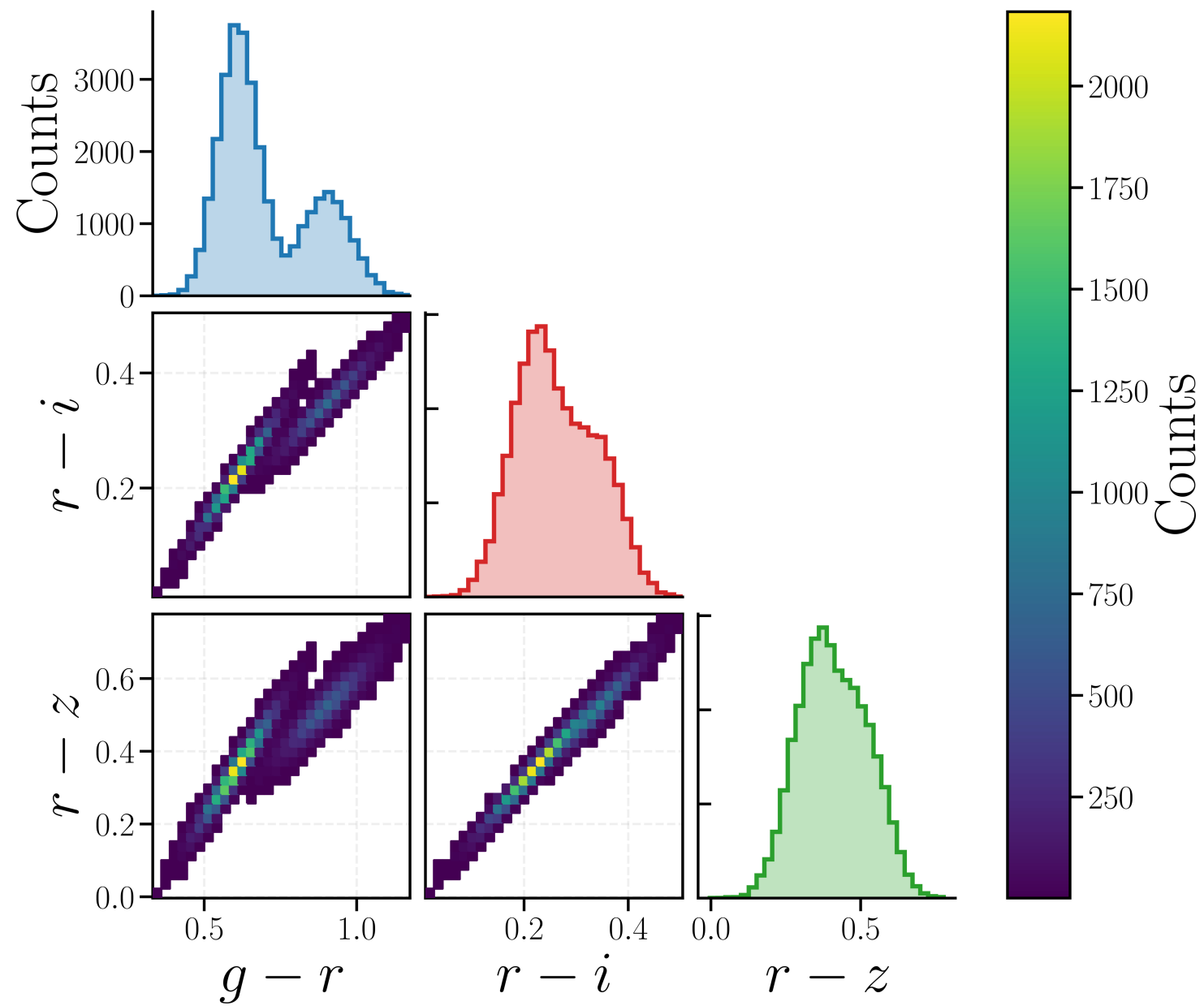
Figure 3. from Joseph Murtagh et al 2026 Astron. J. 171 doi:10.3847/1538-3881/ae27bd https://dx.doi.org/10.3847/1538-3881/ae27bd © 2026. The Author(s). Published by the American Astronomical Society.
