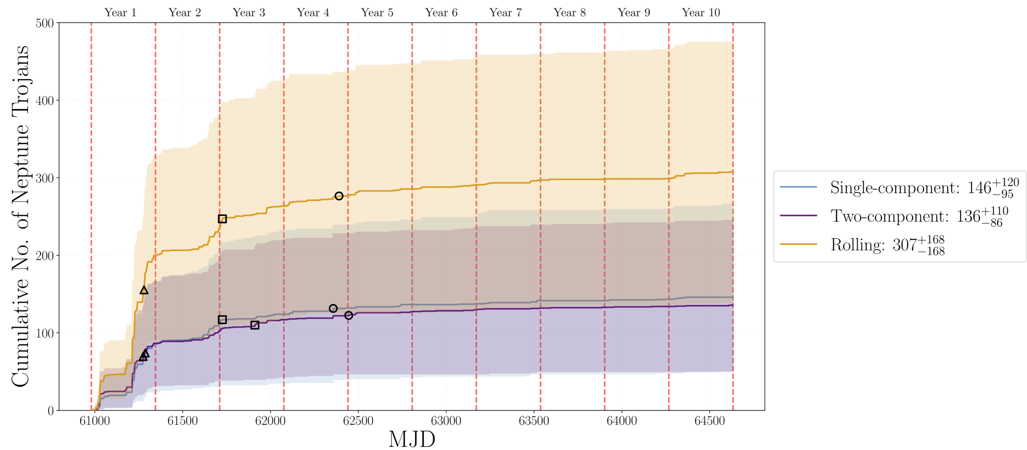
Figure C1. from Joseph Murtagh et al 2026 Astron. J. 171 doi:10.3847/1538-3881/ae27bd https://dx.doi.org/10.3847/1538-3881/ae27bd © 2026. The Author(s). Published by the American Astronomical Society.
