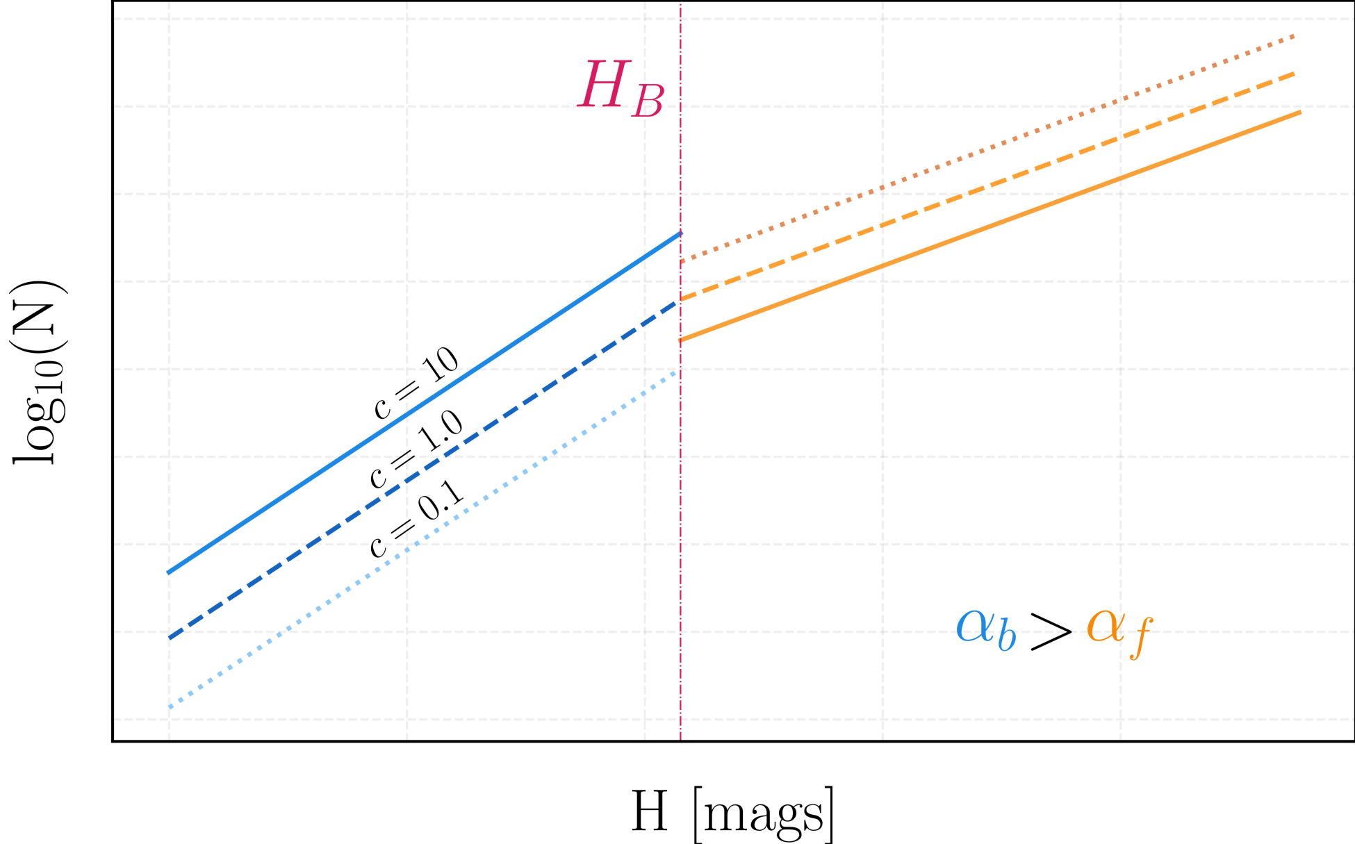
Figure A1. from Joseph Murtagh et al 2026 Astron. J. 171 doi:10.3847/1538-3881/ae27bd https://dx.doi.org/10.3847/1538-3881/ae27bd © 2026. The Author(s). Published by the American Astronomical Society.
