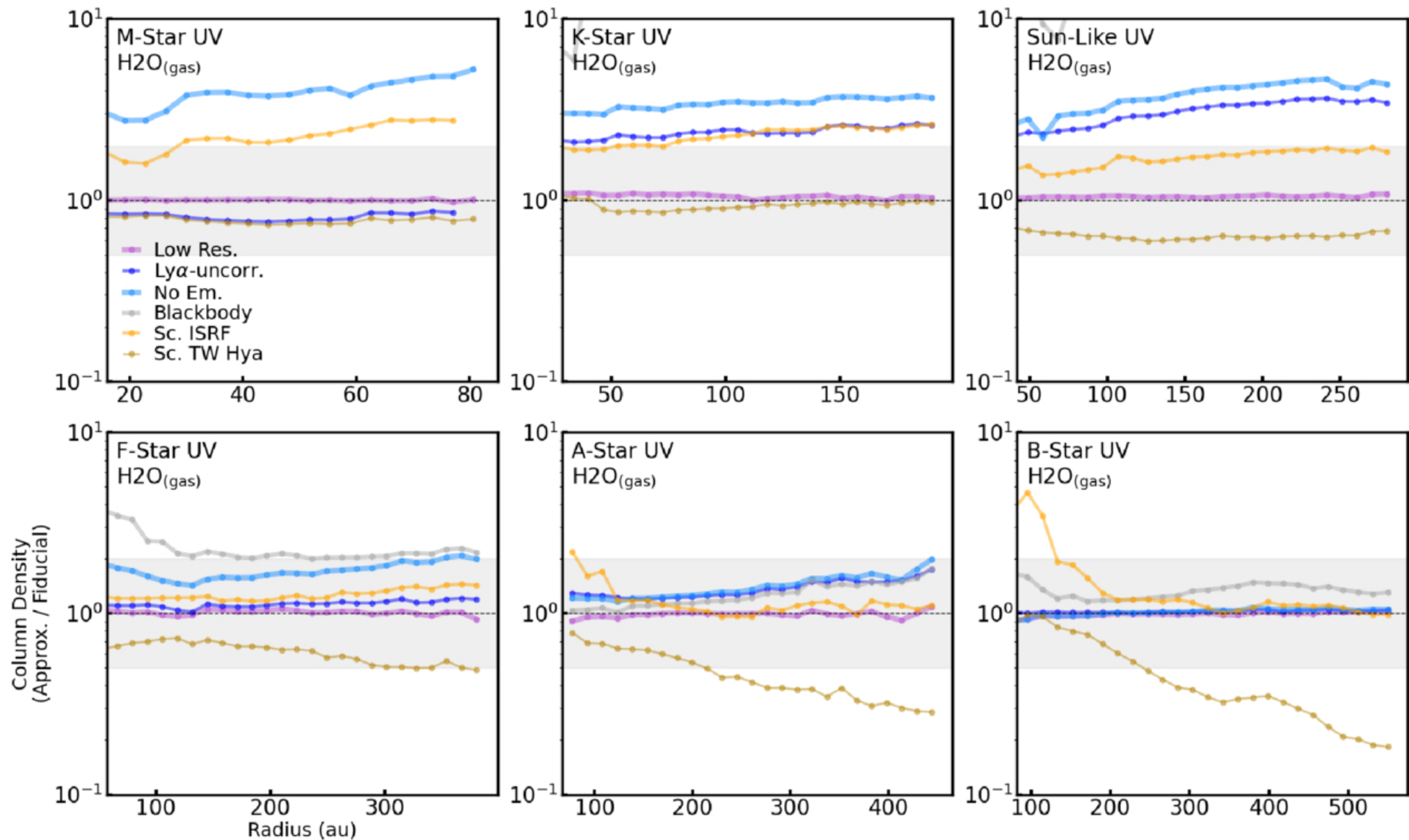
Figure 9. from Jamila Pegues et al 2026 Astron. J. 171 doi:10.3847/1538-3881/ae267a https://dx.doi.org/10.3847/1538-3881/ae267a © 2026. The Author(s). Published by the American Astronomical Society.
