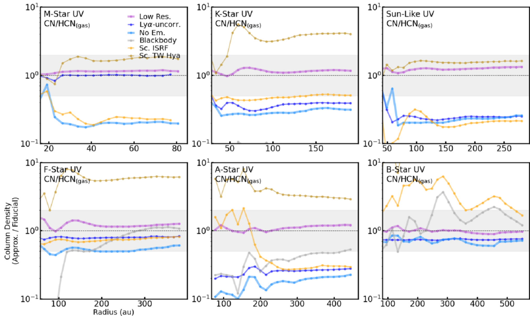
Figure 8. from Jamila Pegues et al 2026 Astron. J. 171 doi:10.3847/1538-3881/ae267a https://dx.doi.org/10.3847/1538-3881/ae267a © 2026. The Author(s). Published by the American Astronomical Society.
