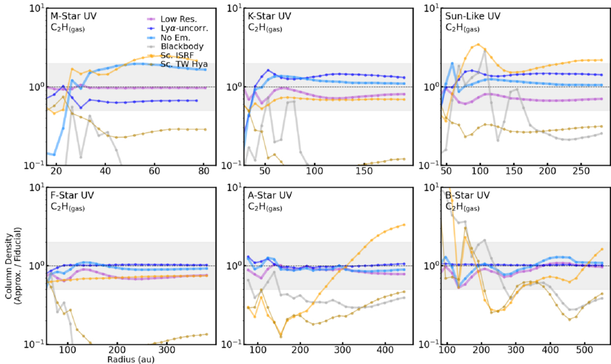
Figure 7. from Jamila Pegues et al 2026 Astron. J. 171 doi:10.3847/1538-3881/ae267a https://dx.doi.org/10.3847/1538-3881/ae267a © 2026. The Author(s). Published by the American Astronomical Society.
