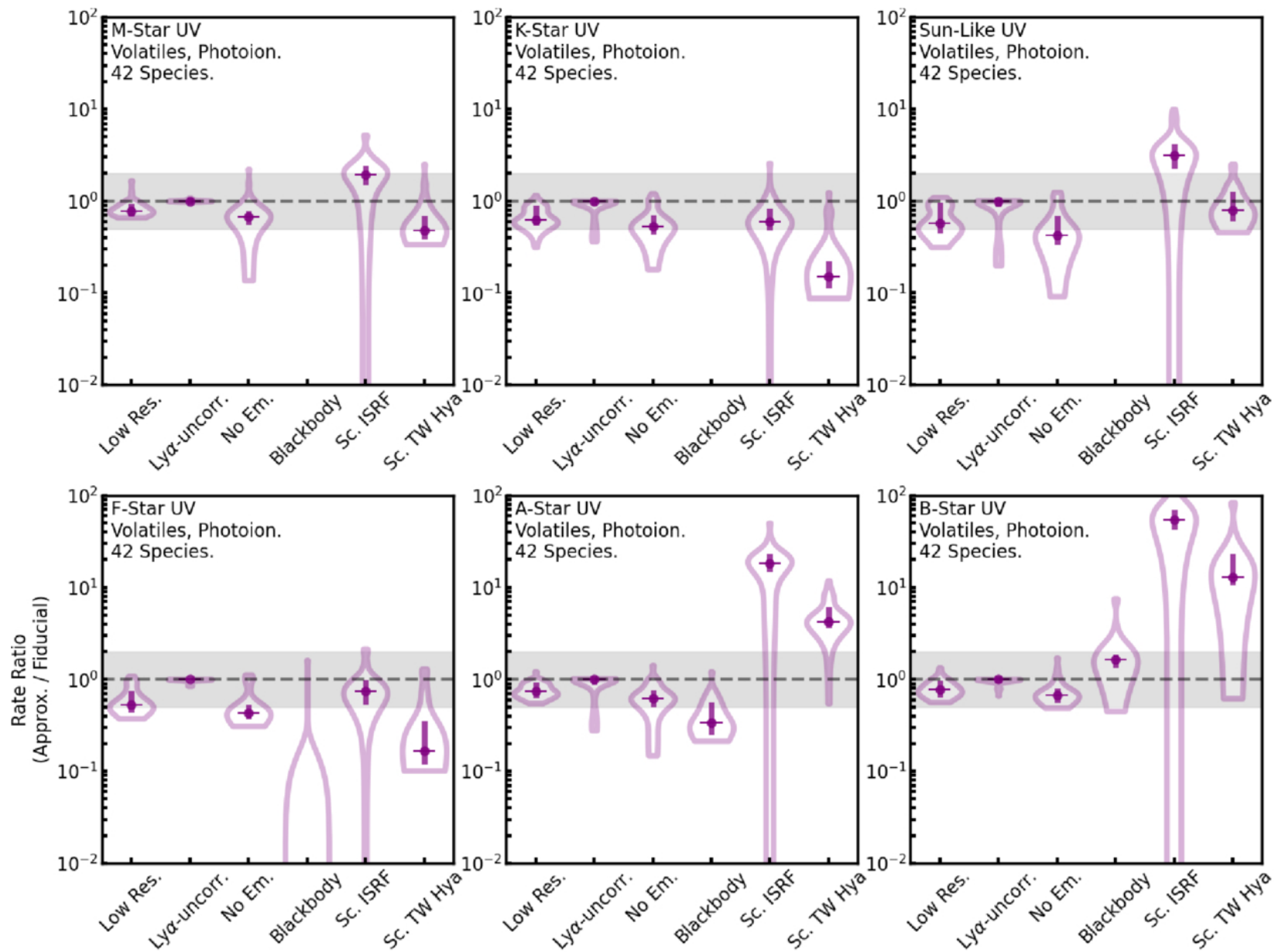
Figure 6. from Jamila Pegues et al 2026 Astron. J. 171 doi:10.3847/1538-3881/ae267a https://dx.doi.org/10.3847/1538-3881/ae267a © 2026. The Author(s). Published by the American Astronomical Society.
