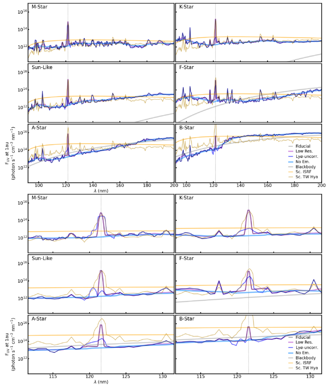
Figure 3. from Jamila Pegues et al 2026 Astron. J. 171 doi:10.3847/1538-3881/ae267a https://dx.doi.org/10.3847/1538-3881/ae267a © 2026. The Author(s). Published by the American Astronomical Society.
