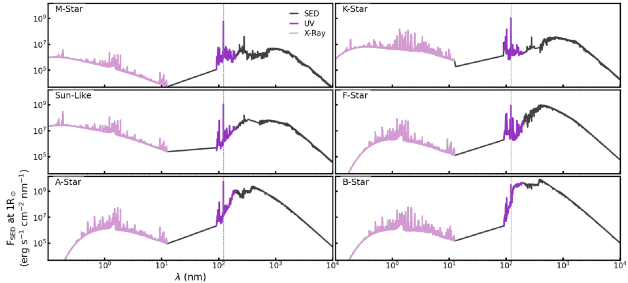
Figure 2. from Jamila Pegues et al 2026 Astron. J. 171 doi:10.3847/1538-3881/ae267a https://dx.doi.org/10.3847/1538-3881/ae267a © 2026. The Author(s). Published by the American Astronomical Society.
