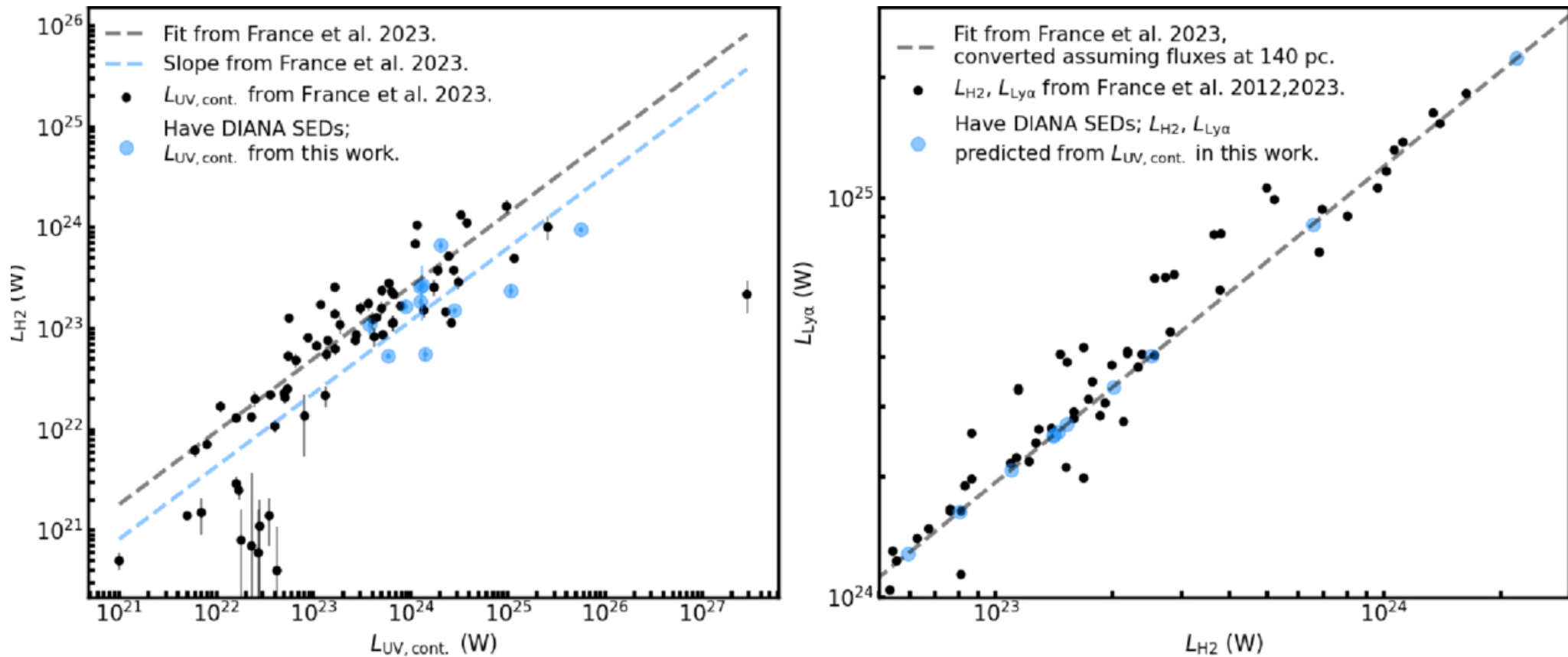
Figure 11. from Jamila Pegues et al 2026 Astron. J. 171 doi:10.3847/1538-3881/ae267a https://dx.doi.org/10.3847/1538-3881/ae267a © 2026. The Author(s). Published by the American Astronomical Society.
