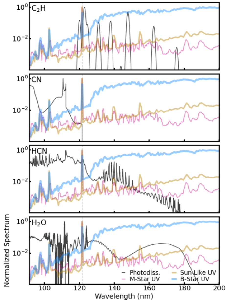
Figure 1. from Jamila Pegues et al 2026 Astron. J. 171 doi:10.3847/1538-3881/ae267a https://dx.doi.org/10.3847/1538-3881/ae267a © 2026. The Author(s). Published by the American Astronomical Society.
