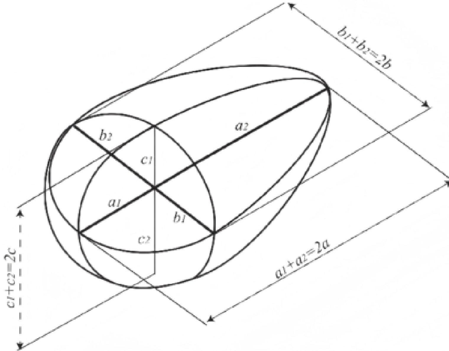
Figure 7. from Xiangyu Fan et al 2026 Astron. J. 171 doi:10.3847/1538-3881/ae2678 https://dx.doi.org/10.3847/1538-3881/ae2678 © 2026. The Author(s). Published by the American Astronomical Society.
