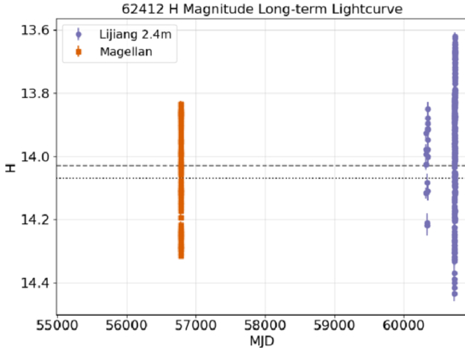
Figure 6. from Xiangyu Fan et al 2026 Astron. J. 171 doi:10.3847/1538-3881/ae2678 https://dx.doi.org/10.3847/1538-3881/ae2678 © 2026. The Author(s). Published by the American Astronomical Society.
