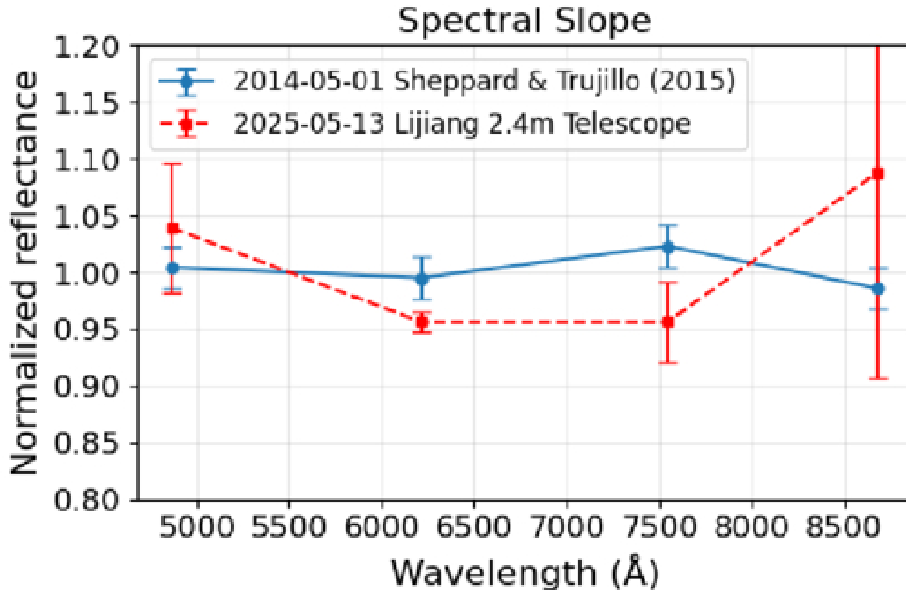
Figure 3. from Xiangyu Fan et al 2026 Astron. J. 171 doi:10.3847/1538-3881/ae2678 https://dx.doi.org/10.3847/1538-3881/ae2678 © 2026. The Author(s). Published by the American Astronomical Society.
