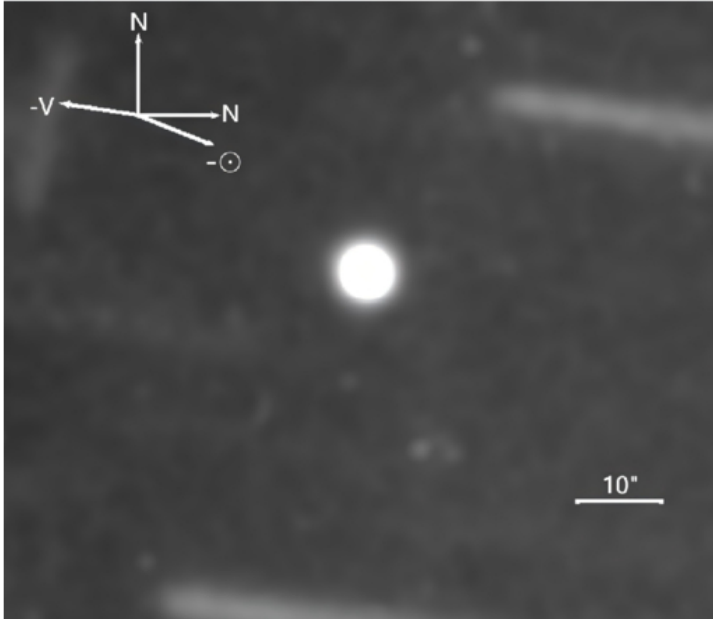
Figure 2. from Xiangyu Fan et al 2026 Astron. J. 171 doi:10.3847/1538-3881/ae2678 https://dx.doi.org/10.3847/1538-3881/ae2678 © 2026. The Author(s). Published by the American Astronomical Society.
