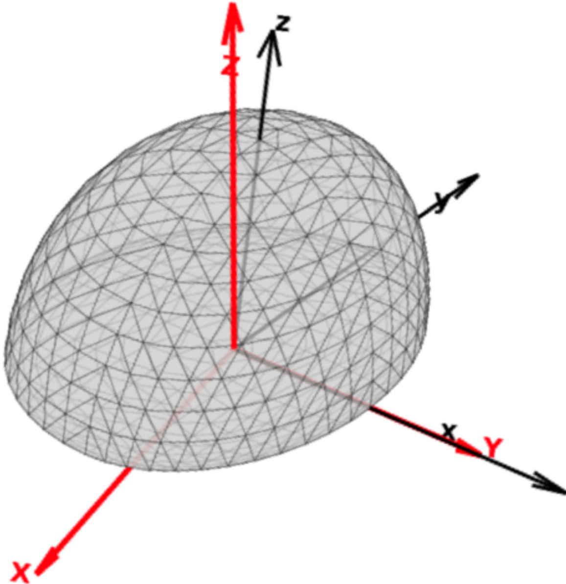
Figure 11. from Xiangyu Fan et al 2026 Astron. J. 171 doi:10.3847/1538-3881/ae2678 https://dx.doi.org/10.3847/1538-3881/ae2678 © 2026. The Author(s). Published by the American Astronomical Society.
