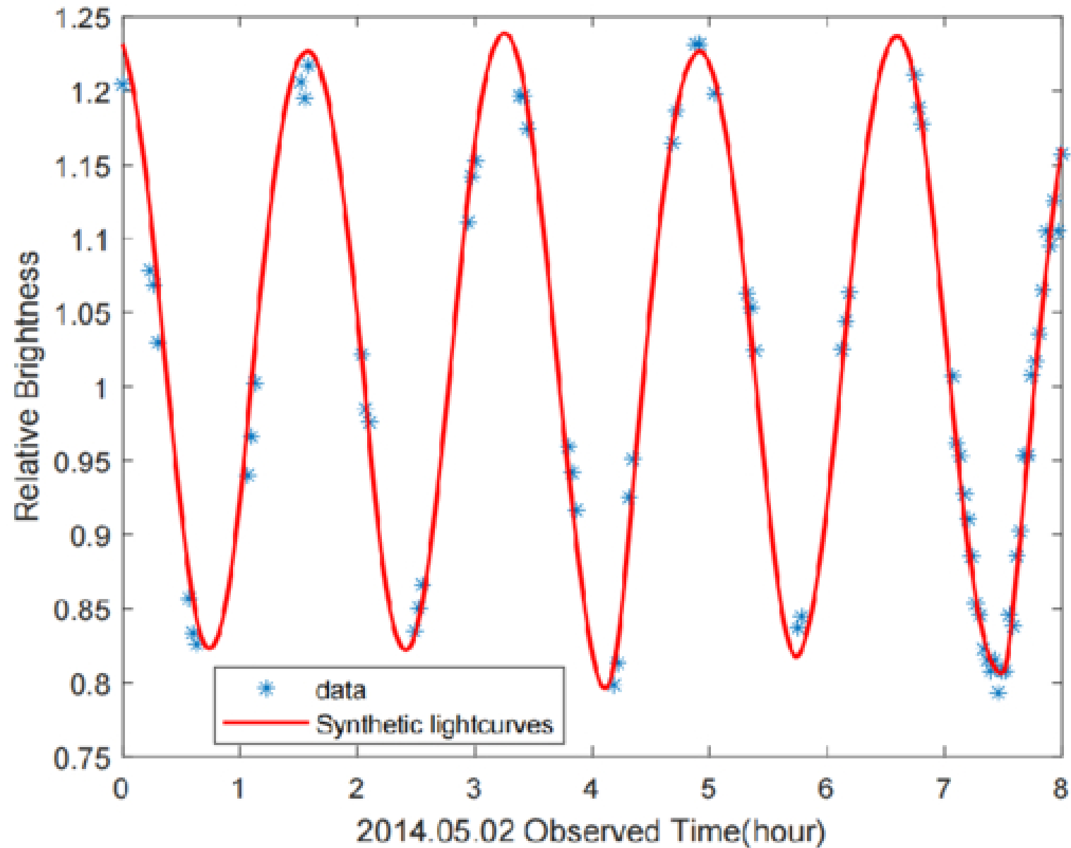
Figure 10. from Xiangyu Fan et al 2026 Astron. J. 171 doi:10.3847/1538-3881/ae2678 https://dx.doi.org/10.3847/1538-3881/ae2678 © 2026. The Author(s). Published by the American Astronomical Society.
