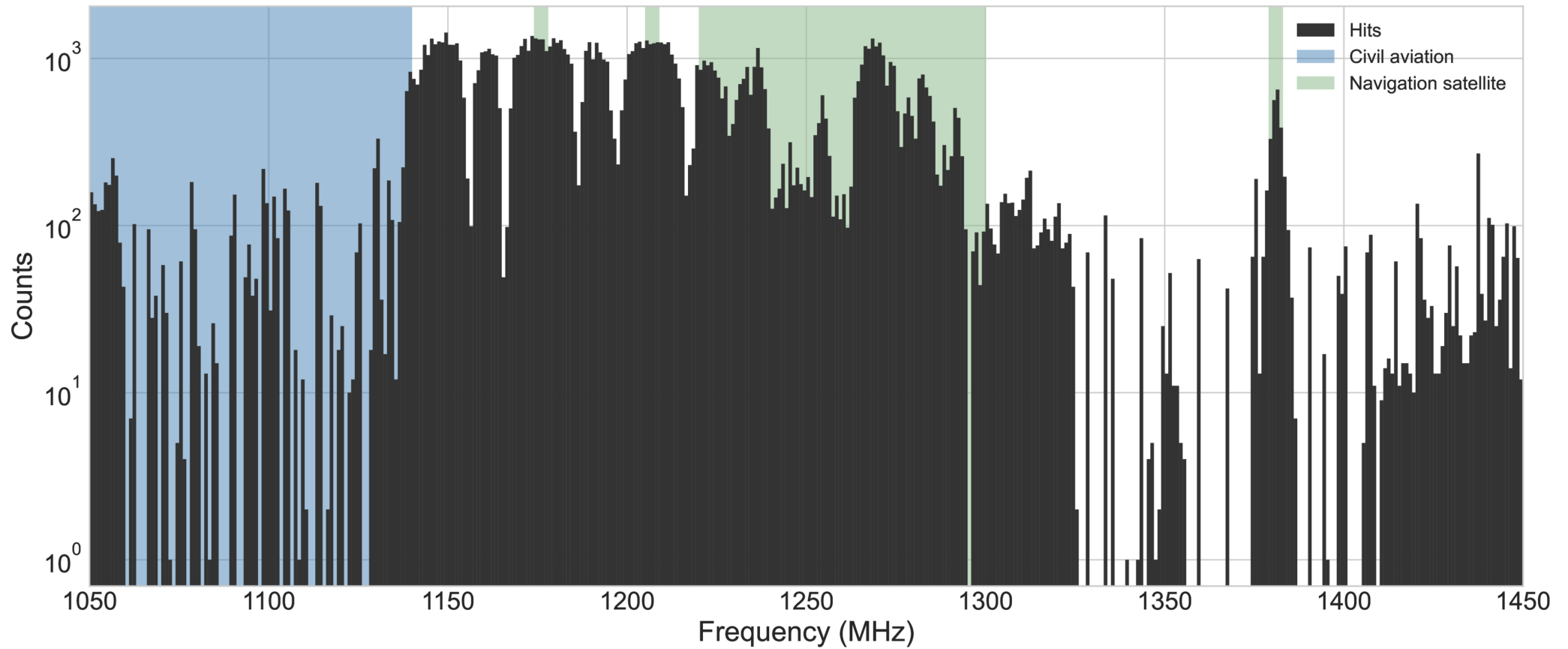
Figure 3. from Bo-Lun Huang et al 2026 Astron. J. 171 doi:10.3847/1538-3881/ae2470 https://dx.doi.org/10.3847/1538-3881/ae2470 © 2025. The Author(s). Published by the American Astronomical Society.
