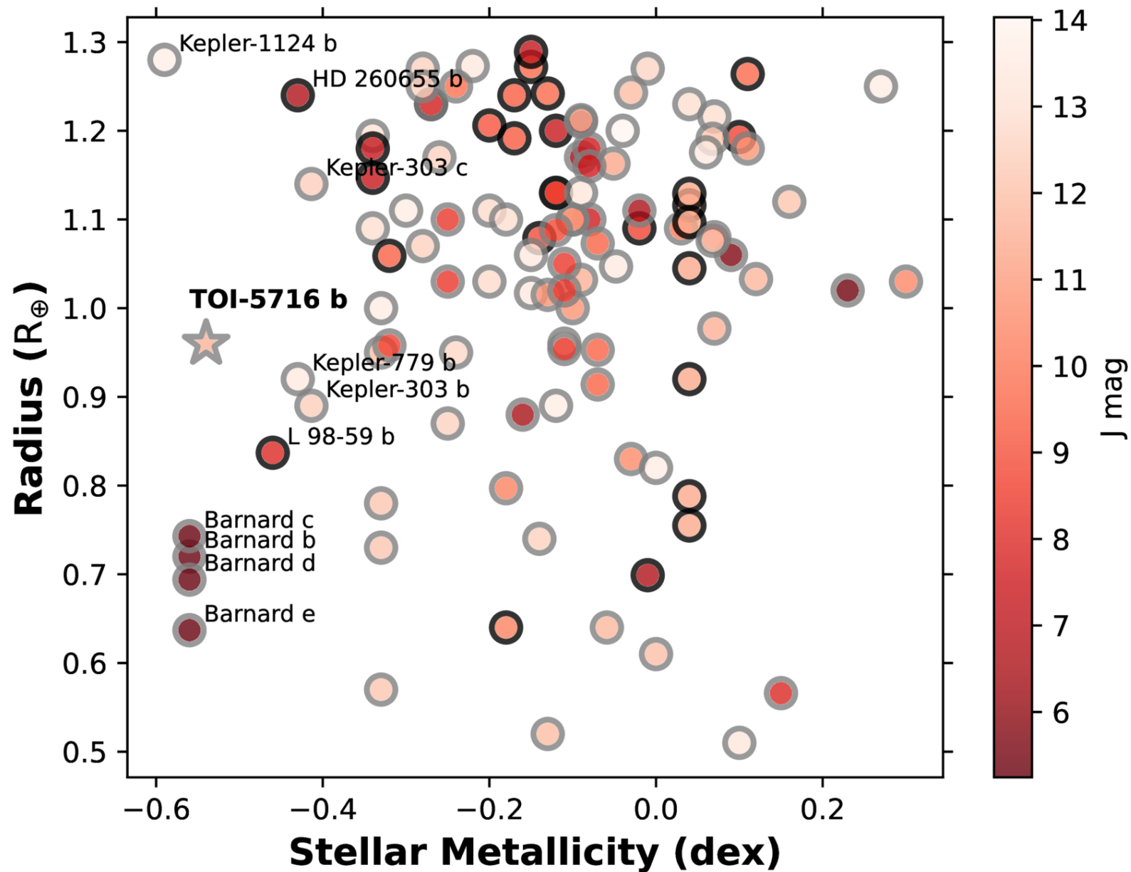
Figure 5. from Jonathan Gomez Barrientos et al 2026 Astron. J. 171 doi:10.3847/1538-3881/ae246f https://dx.doi.org/10.3847/1538-3881/ae246f © 2026. The Author(s). Published by the American Astronomical Society.
