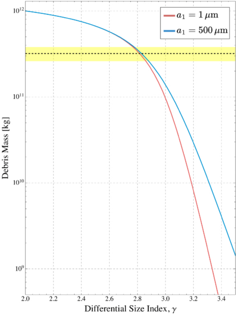
Figure 2. from Salvatore A. Cordova Quijano et al 2026 Astron. J. 171 doi:10.3847/1538-3881/ae2450 https://dx.doi.org/10.3847/1538-3881/ae2450 © 2026. The Author(s). Published by the American Astronomical Society.
