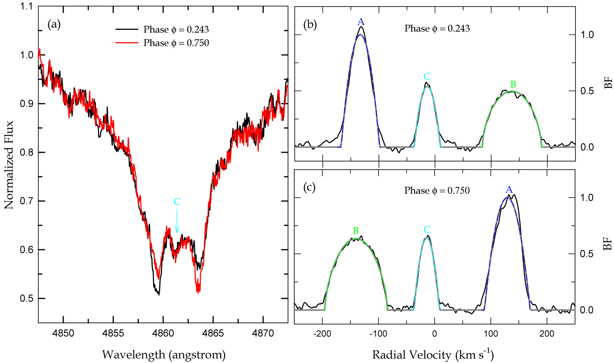
Figure 3. from Jae Woo Lee et al 2026 Astron. J. 171 doi:10.3847/1538-3881/ae23ce https://dx.doi.org/10.3847/1538-3881/ae23ce © 2025. The Author(s). Published by the American Astronomical Society.
