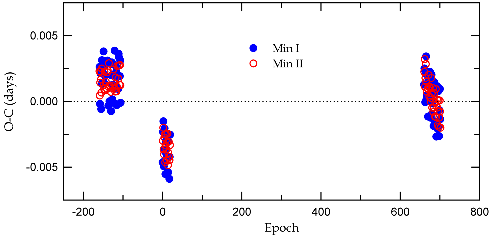
Figure 2. from Jae Woo Lee et al 2026 Astron. J. 171 doi:10.3847/1538-3881/ae23ce https://dx.doi.org/10.3847/1538-3881/ae23ce © 2025. The Author(s). Published by the American Astronomical Society.
