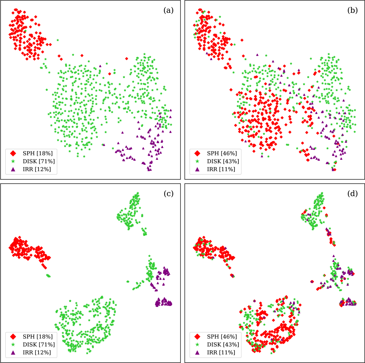
Figure 7. from Guanwen Fang et al 2026 Astron. J. 171 doi:10.3847/1538-3881/ae2324 https://dx.doi.org/10.3847/1538-3881/ae2324 © 2026. The Author(s). Published by the American Astronomical Society.
