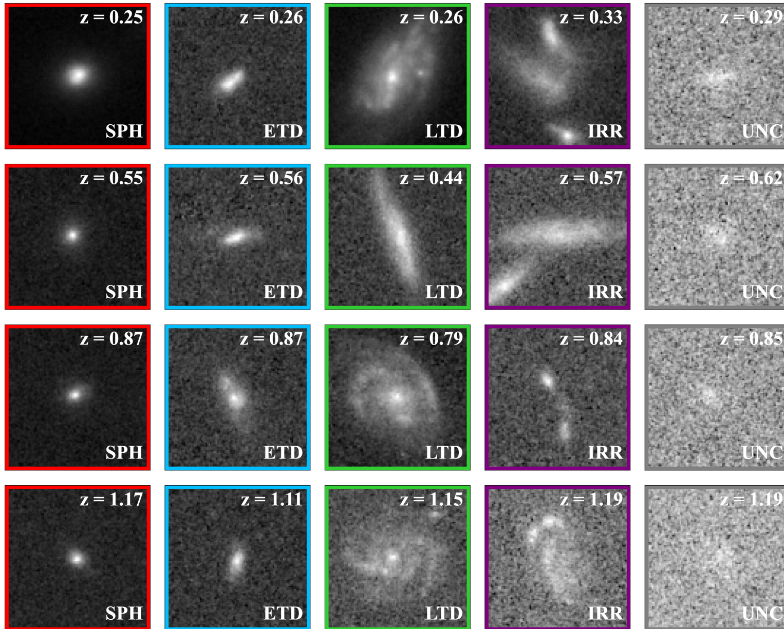
Figure 6. from Guanwen Fang et al 2026 Astron. J. 171 doi:10.3847/1538-3881/ae2324 https://dx.doi.org/10.3847/1538-3881/ae2324 © 2026. The Author(s). Published by the American Astronomical Society.
