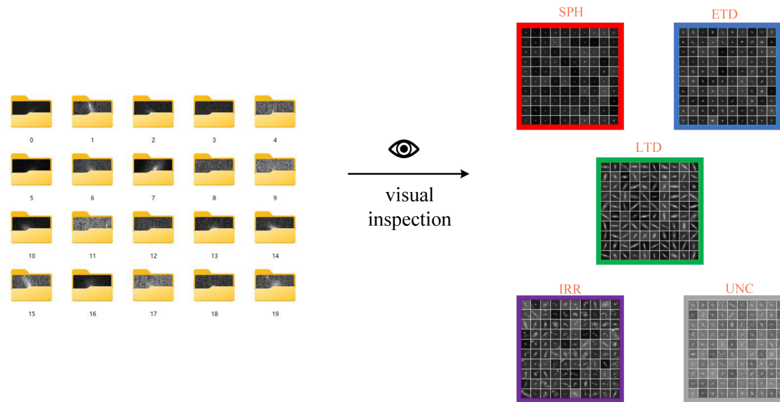
Figure 5. from Guanwen Fang et al 2026 Astron. J. 171 doi:10.3847/1538-3881/ae2324 https://dx.doi.org/10.3847/1538-3881/ae2324 © 2026. The Author(s). Published by the American Astronomical Society.
