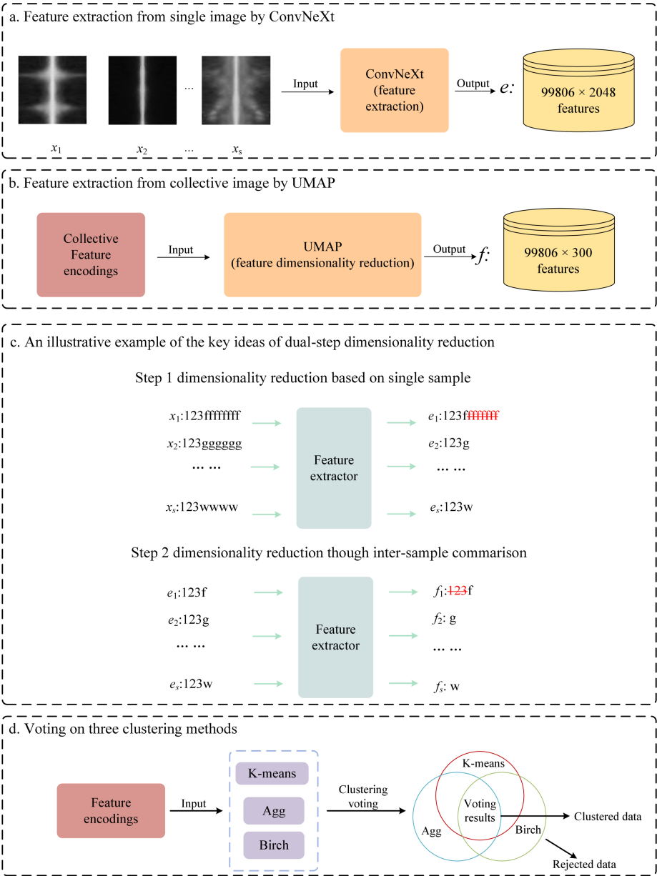
Figure 4. from Guanwen Fang et al 2026 Astron. J. 171 doi:10.3847/1538-3881/ae2324 https://dx.doi.org/10.3847/1538-3881/ae2324 © 2026. The Author(s). Published by the American Astronomical Society.
