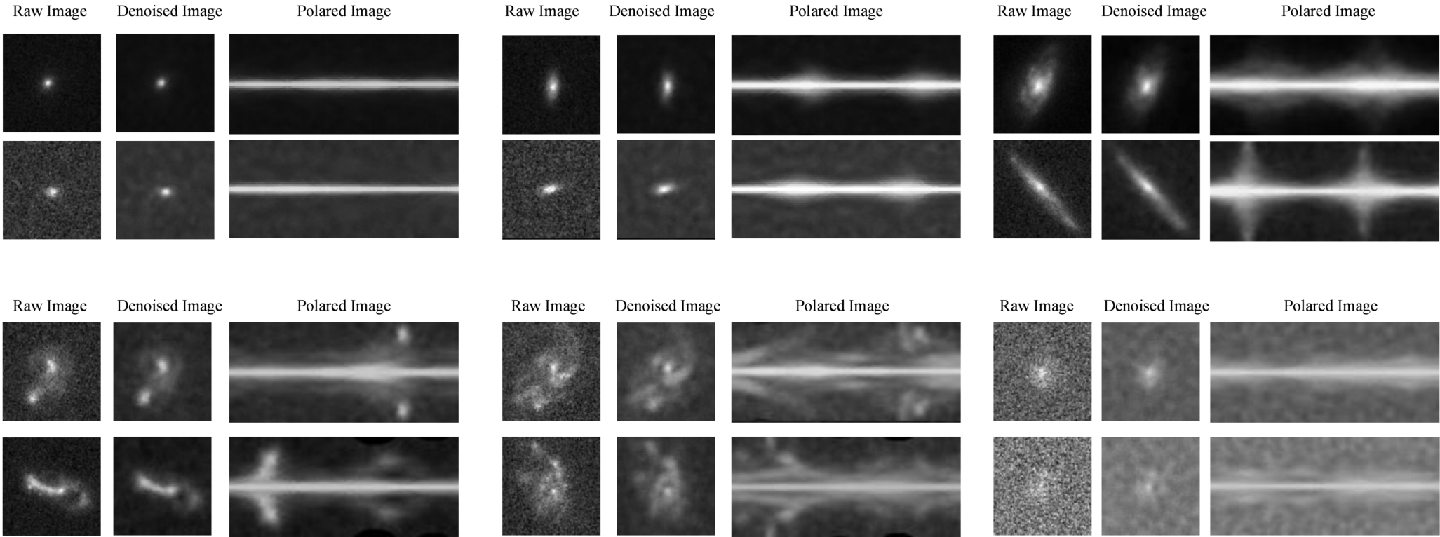
Figure 2. from Guanwen Fang et al 2026 Astron. J. 171 doi:10.3847/1538-3881/ae2324 https://dx.doi.org/10.3847/1538-3881/ae2324 © 2026. The Author(s). Published by the American Astronomical Society.
