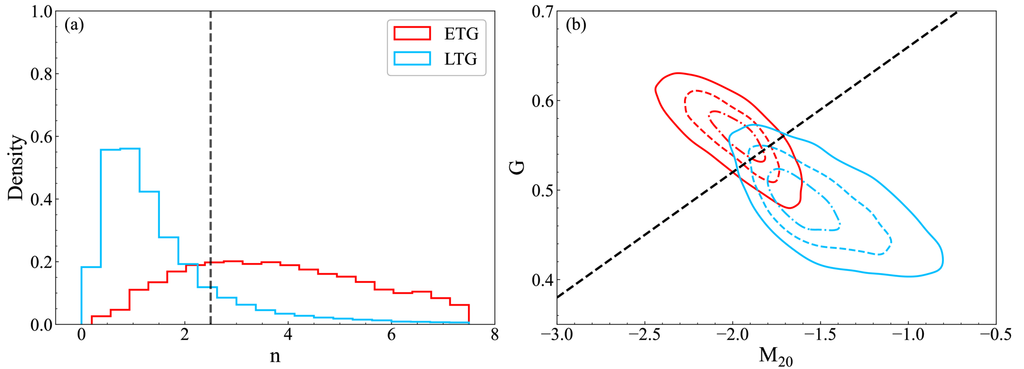
Figure 12. from Guanwen Fang et al 2026 Astron. J. 171 doi:10.3847/1538-3881/ae2324 https://dx.doi.org/10.3847/1538-3881/ae2324 © 2026. The Author(s). Published by the American Astronomical Society.
