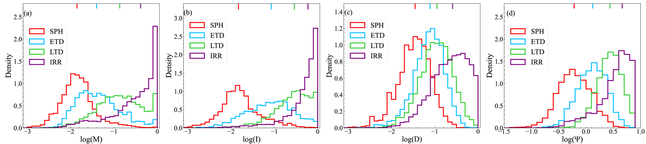
Figure 11. from Guanwen Fang et al 2026 Astron. J. 171 doi:10.3847/1538-3881/ae2324 https://dx.doi.org/10.3847/1538-3881/ae2324 © 2026. The Author(s). Published by the American Astronomical Society.
