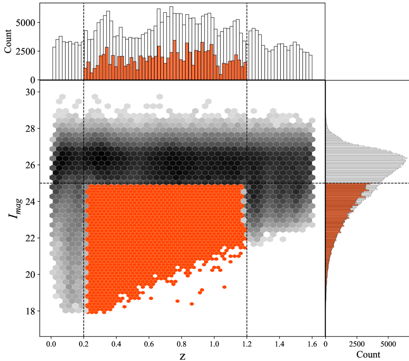
Figure 1. from Guanwen Fang et al 2026 Astron. J. 171 doi:10.3847/1538-3881/ae2324 https://dx.doi.org/10.3847/1538-3881/ae2324 © 2026. The Author(s). Published by the American Astronomical Society.
