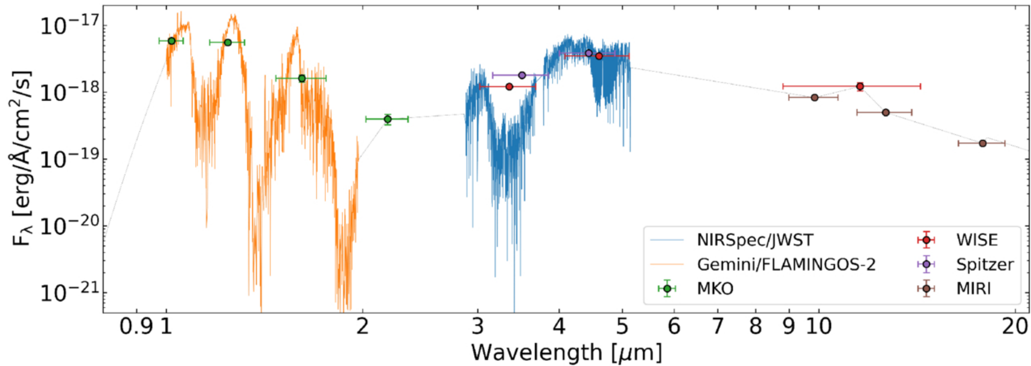
Figure 9. from Rocio Kiman et al 2026 Astron. J. 171 doi:10.3847/1538-3881/ae230f https://dx.doi.org/10.3847/1538-3881/ae230f © 2026. The Author(s). Published by the American Astronomical Society.
