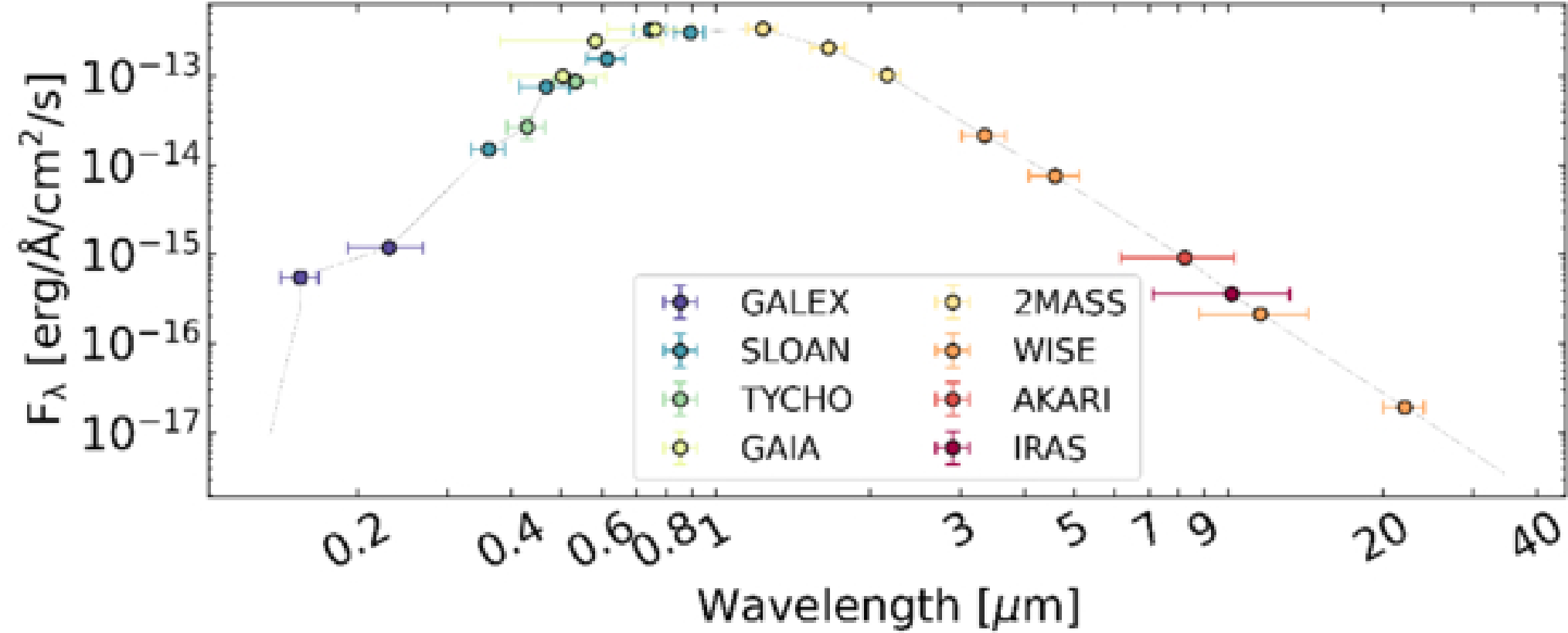
Figure 8. from Rocio Kiman et al 2026 Astron. J. 171 doi:10.3847/1538-3881/ae230f https://dx.doi.org/10.3847/1538-3881/ae230f © 2026. The Author(s). Published by the American Astronomical Society.
