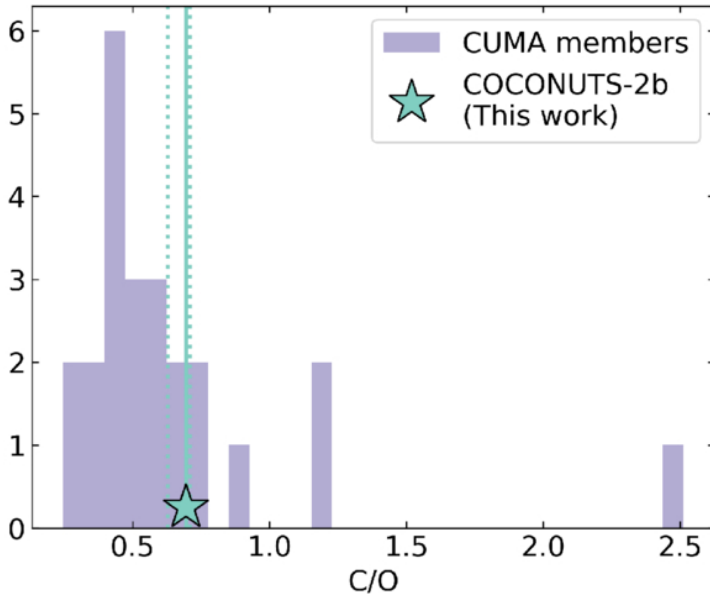
Figure 6. from Rocio Kiman et al 2026 Astron. J. 171 doi:10.3847/1538-3881/ae230f https://dx.doi.org/10.3847/1538-3881/ae230f © 2026. The Author(s). Published by the American Astronomical Society.
