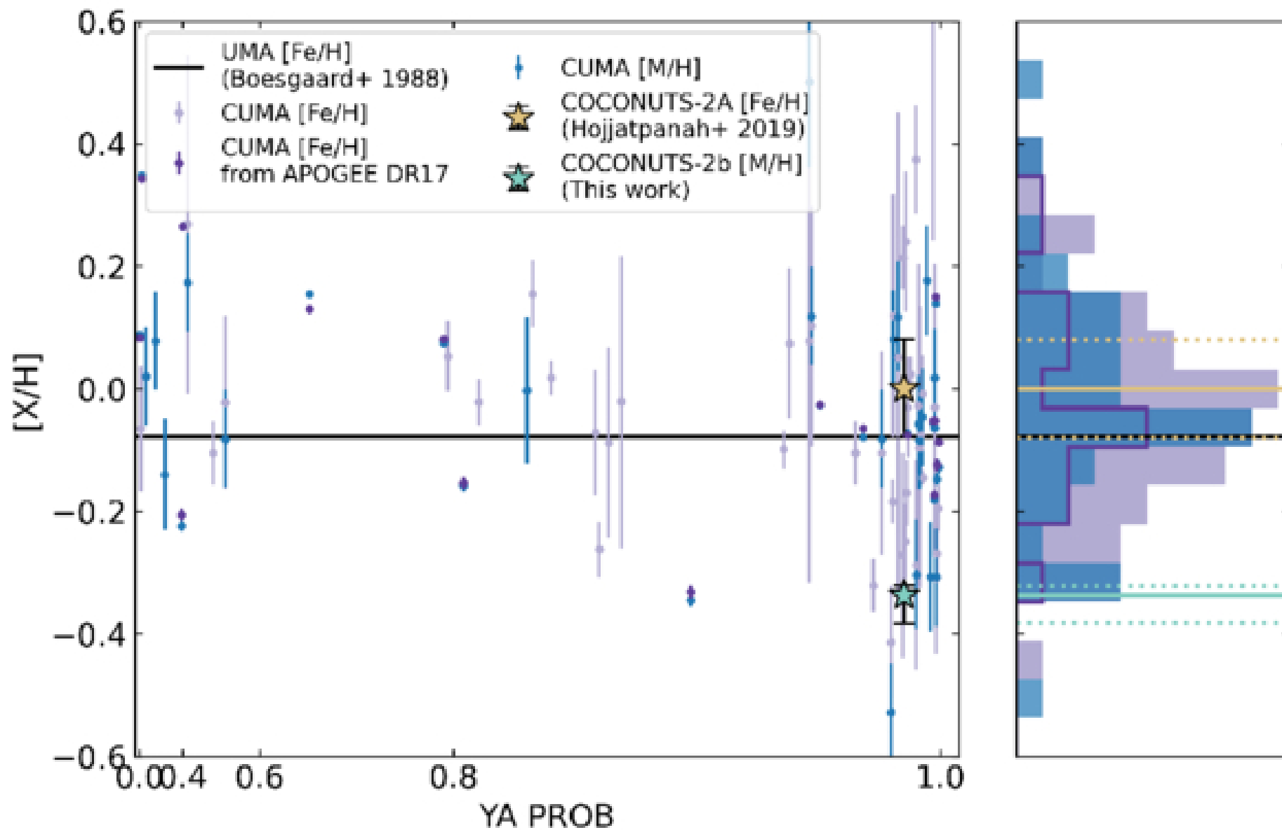
Figure 5. from Rocio Kiman et al 2026 Astron. J. 171 doi:10.3847/1538-3881/ae230f https://dx.doi.org/10.3847/1538-3881/ae230f © 2026. The Author(s). Published by the American Astronomical Society.
