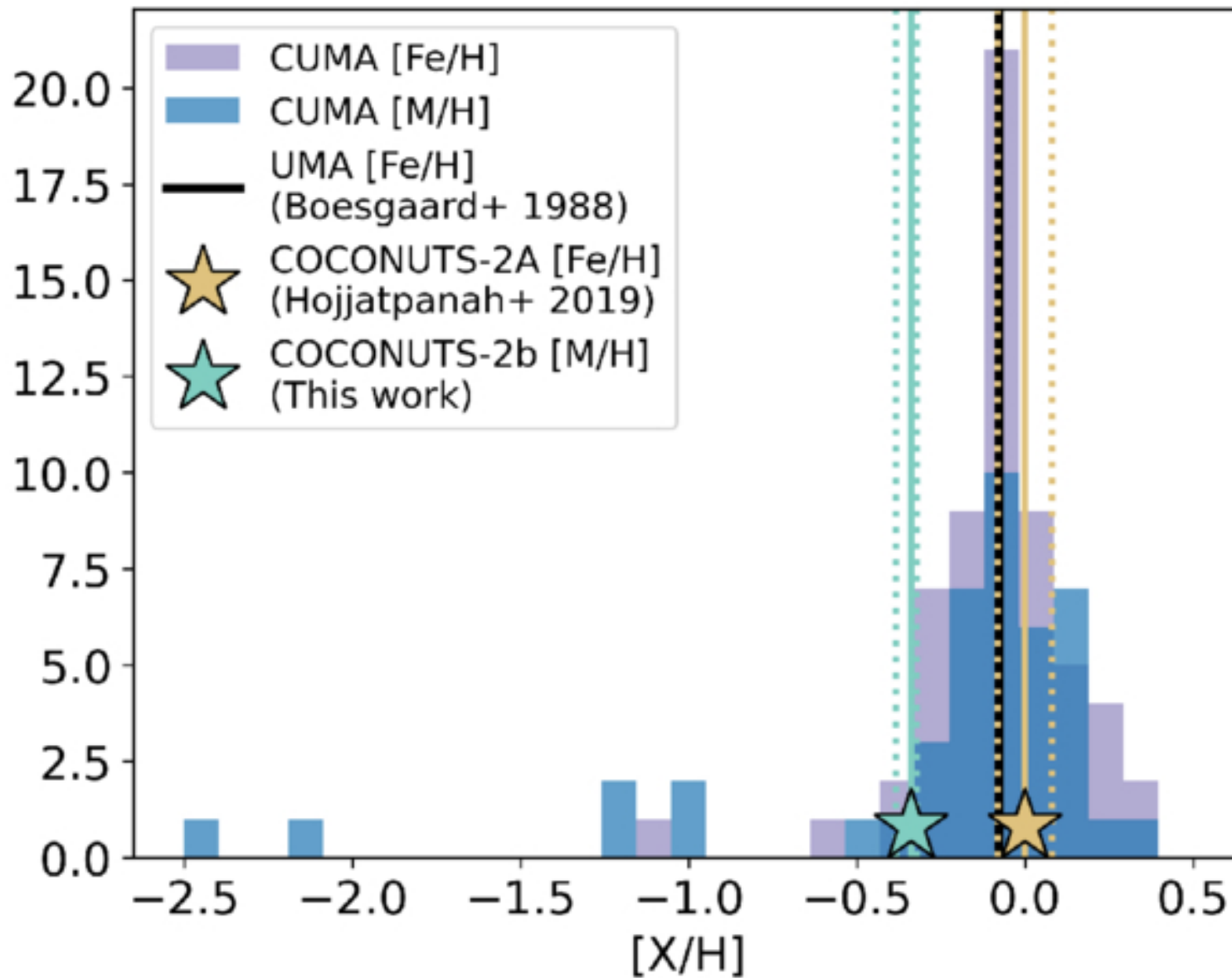
Figure 4. from Rocio Kiman et al 2026 Astron. J. 171 doi:10.3847/1538-3881/ae230f https://dx.doi.org/10.3847/1538-3881/ae230f © 2026. The Author(s). Published by the American Astronomical Society.
