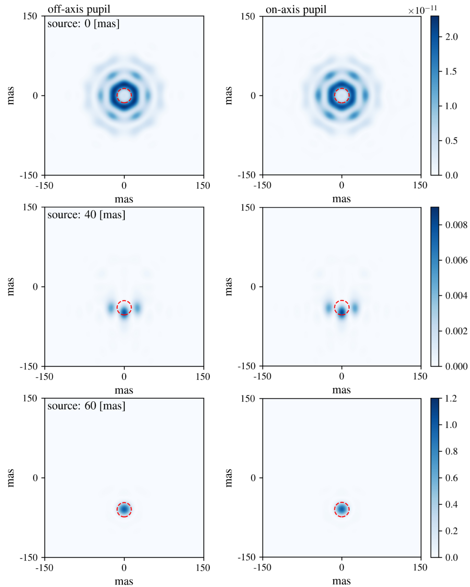
Figure 9. from Jamila S. Taaki et al 2026 Astron. J. 171 doi:10.3847/1538-3881/ae22f1 https://dx.doi.org/10.3847/1538-3881/ae22f1 © 2025. The Author(s). Published by the American Astronomical Society.
