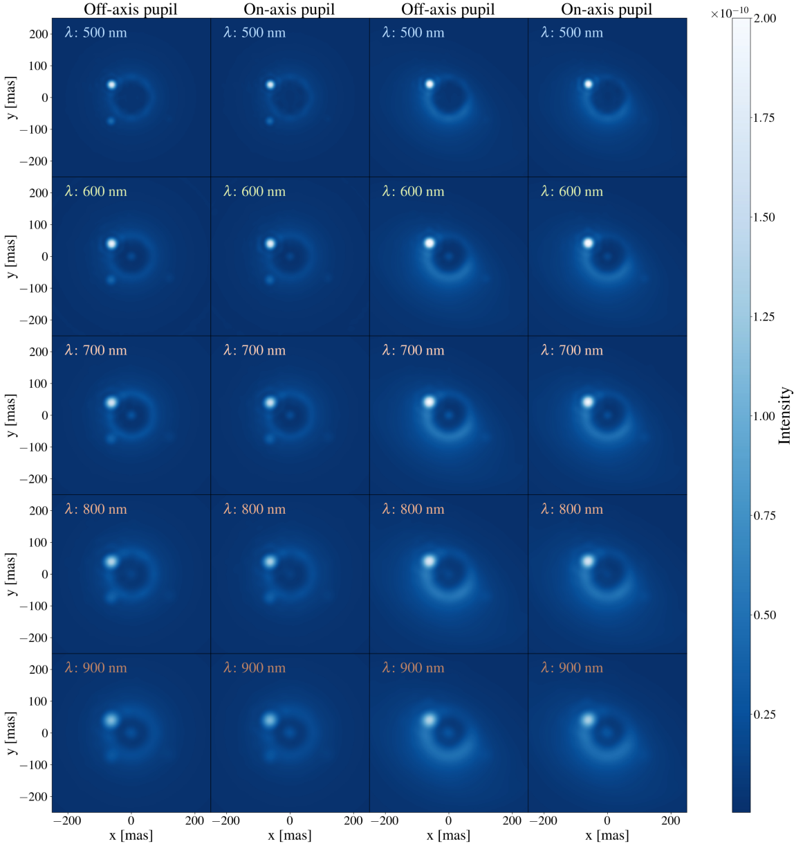
Figure 7. from Jamila S. Taaki et al 2026 Astron. J. 171 doi:10.3847/1538-3881/ae22f1 https://dx.doi.org/10.3847/1538-3881/ae22f1 © 2025. The Author(s). Published by the American Astronomical Society.
