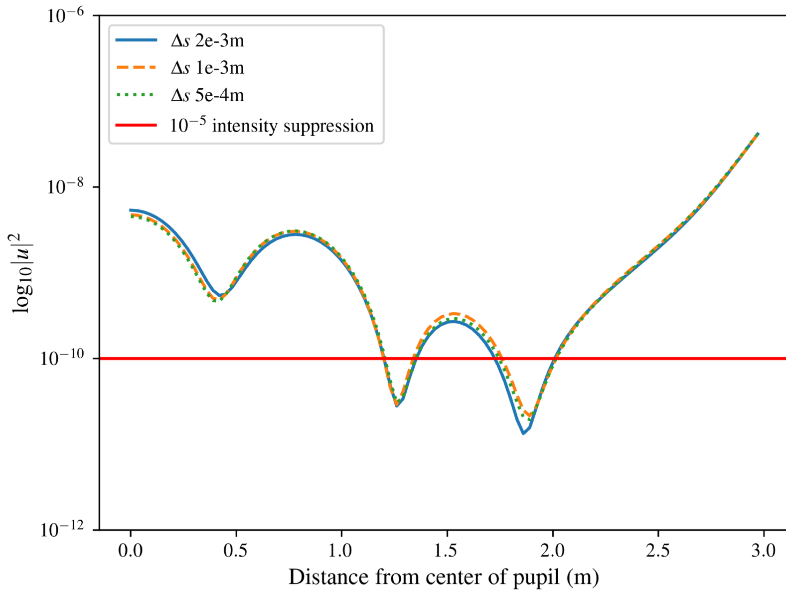
Figure 5. from Jamila S. Taaki et al 2026 Astron. J. 171 doi:10.3847/1538-3881/ae22f1 https://dx.doi.org/10.3847/1538-3881/ae22f1 © 2025. The Author(s). Published by the American Astronomical Society.
