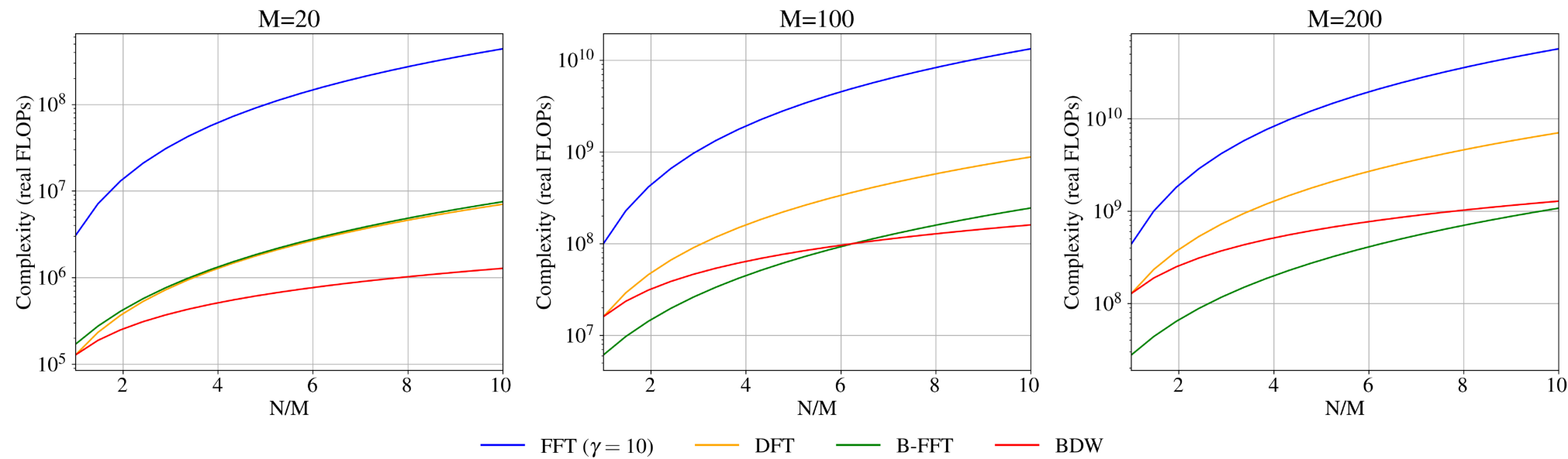
Figure 4. from Jamila S. Taaki et al 2026 Astron. J. 171 doi:10.3847/1538-3881/ae22f1 https://dx.doi.org/10.3847/1538-3881/ae22f1 © 2025. The Author(s). Published by the American Astronomical Society.
