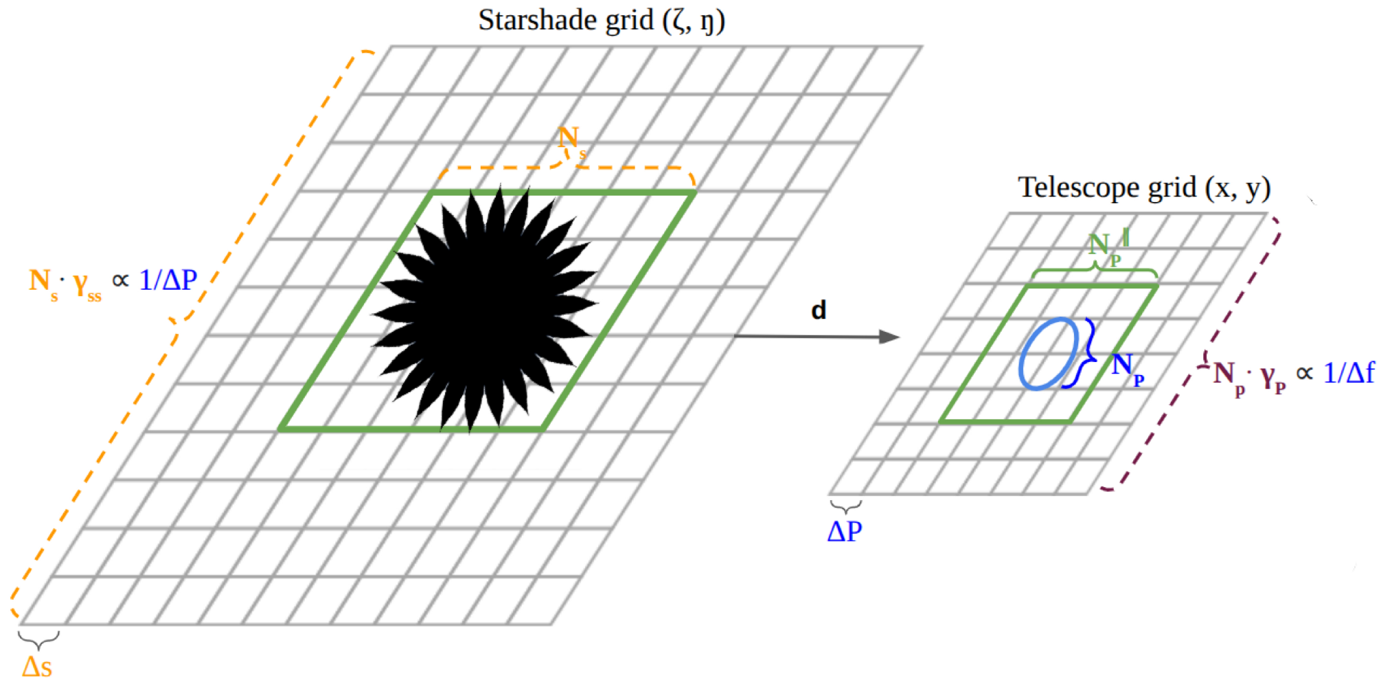
Figure 3. from Jamila S. Taaki et al 2026 Astron. J. 171 doi:10.3847/1538-3881/ae22f1 https://dx.doi.org/10.3847/1538-3881/ae22f1 © 2025. The Author(s). Published by the American Astronomical Society.
