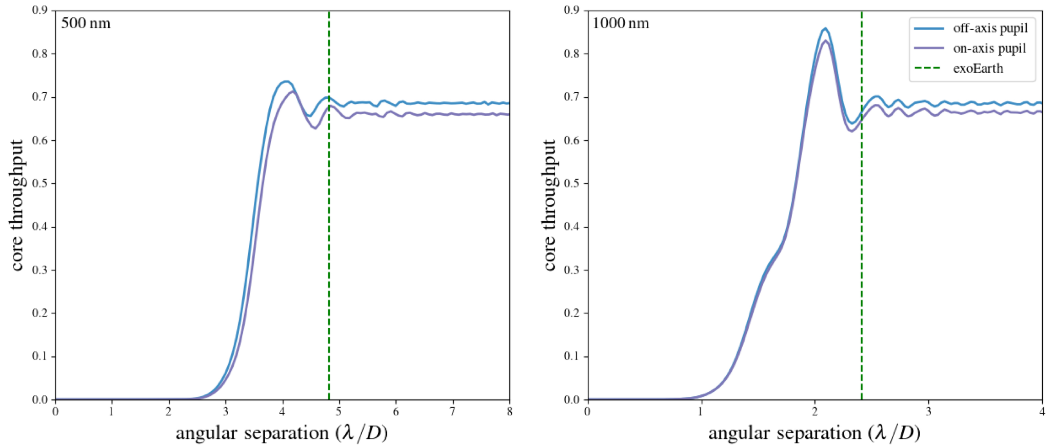
Figure 10. from Jamila S. Taaki et al 2026 Astron. J. 171 doi:10.3847/1538-3881/ae22f1 https://dx.doi.org/10.3847/1538-3881/ae22f1 © 2025. The Author(s). Published by the American Astronomical Society.
